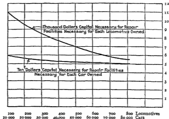
FIG 1—Showing desirable relation of repair facilities to equipment owned 1
